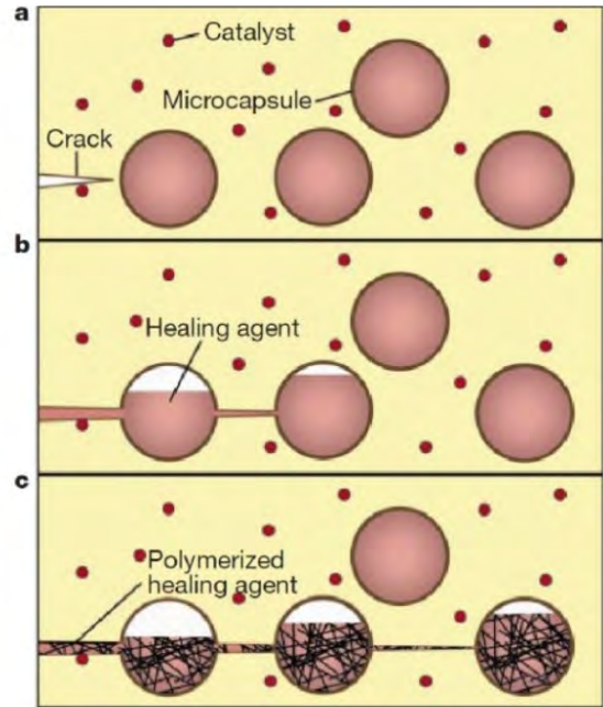
The autonomic healing concept (White et al. 2001).
